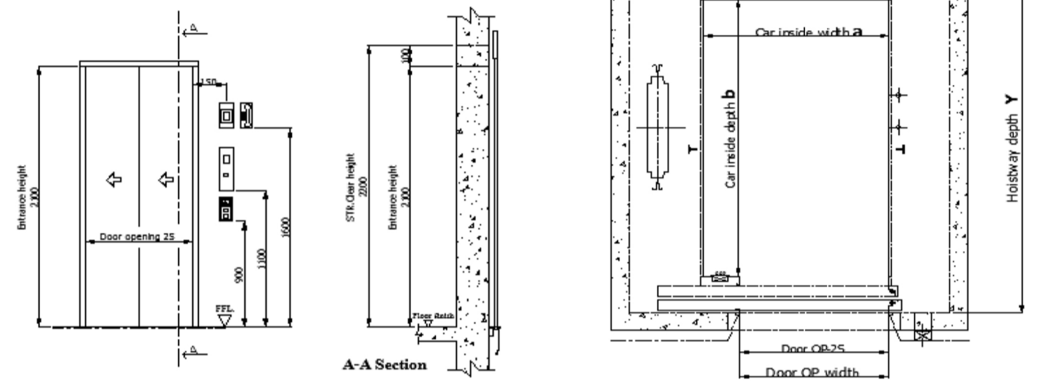
Entrance details (For 2 panel Slide- door) Unit :mm
