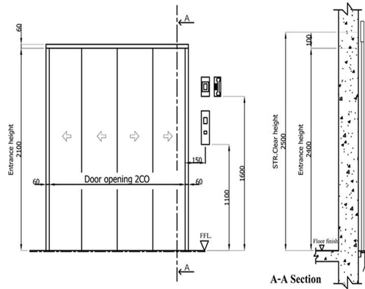
Entrance details (For 4 panel center opening door) Unit :mm
